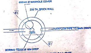
PLAN OF ABSORPTION PIT (NOT TO SCALE)
